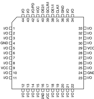
TQFP Top View
