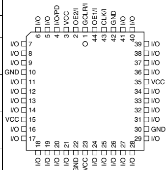
PLCC Top View
