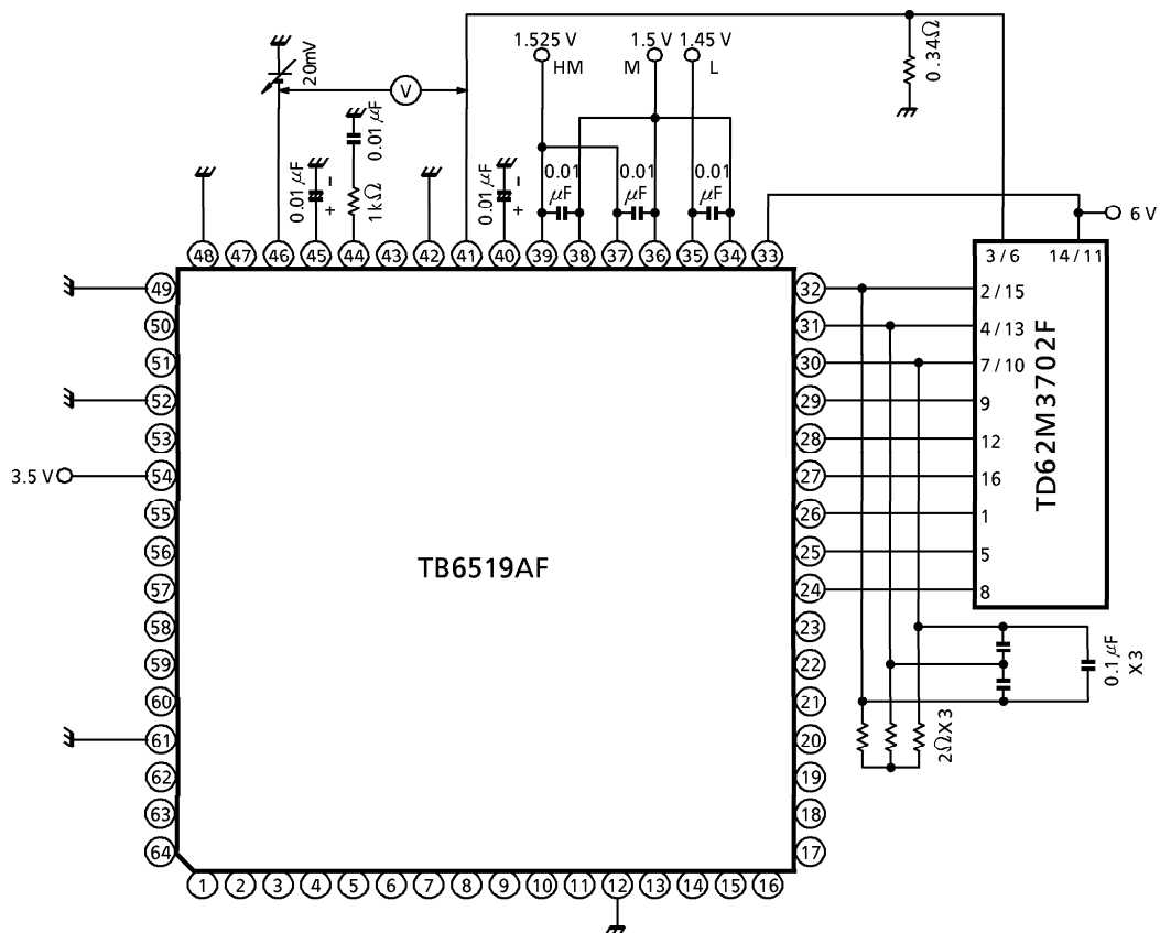
TEST CIRCUIT 16. TLofs
