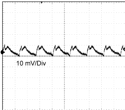
Figure 37. Output Ripple
