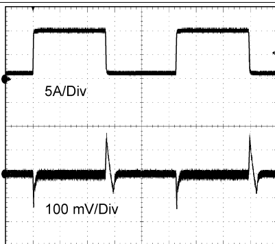
Figure 39. Transient Response
