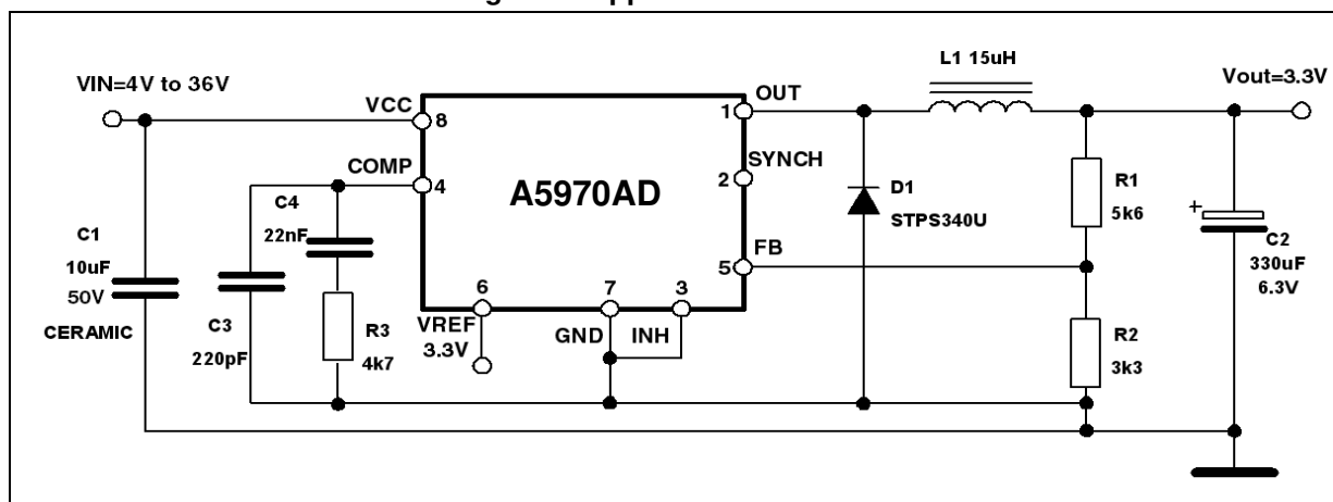
Figure 1. Application schematic
