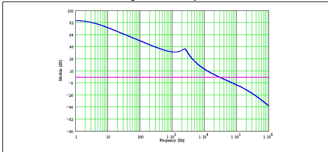
Figure 11. Module plot
