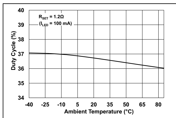
FIGURE 2-9: Duty Cycle vs. Ambient Temperature.
