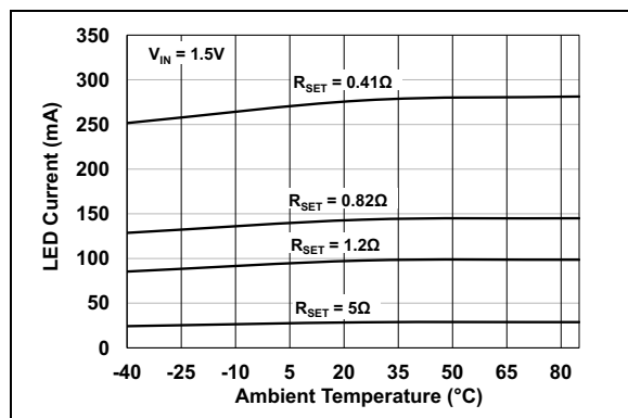
FIGURE 2-7: One White I_{LED} vs. Ambient Temperature.
