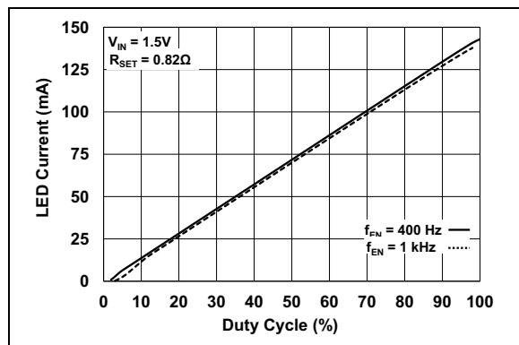
FIGURE 2-8: I_{LED} vs. V_{EN} Duty Cycle.
