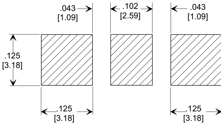
1. INDUCTANCE TO BE 0.1 \mu H MINIMUM. 2. PACKAGE: BULK OR BLISTER TAPE TO IEC-60286-3 TYPE II AND EIA-481-A. 3. TUSONIX STANDARD PART NUMBER: 4700-005. TUSONIX RoHS COMPLIANT PART NUMBER: 4700-005 LF. CUSTOMER MUST SPECIFY STANDARD OR RoHS PART NUMBER WHEN ORDERING. 4. PART MARKING: STANDARD PART: NO MARKING. RoHS PART: LABELED ON PACKAGING ONLY. 5. ELECTRODE TERMINATION: STANDARD 60/40 SOLDER; RoHS COMPLIANT - MATTE TIN.
