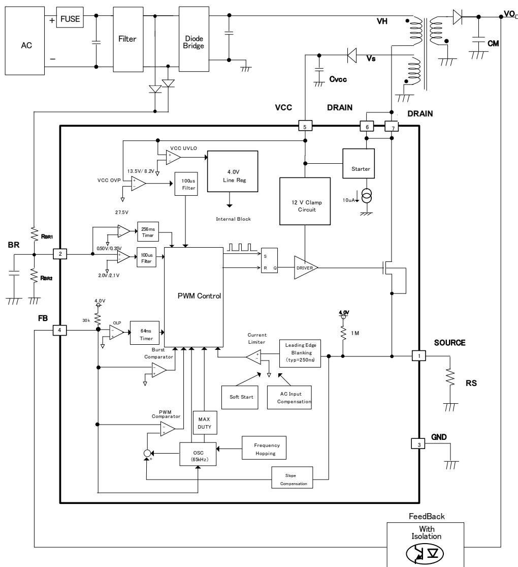
Figure 3. Block Diagram
