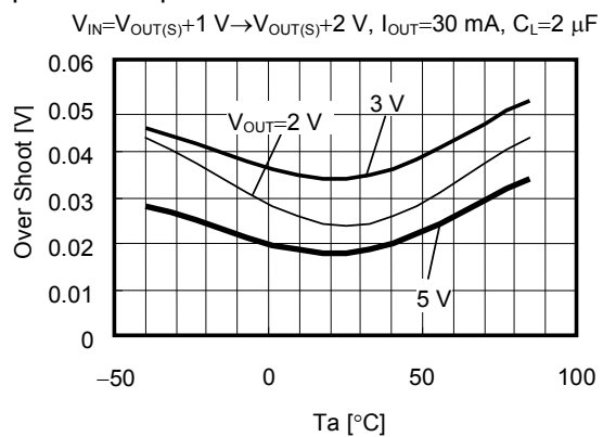
Temperature dependence
