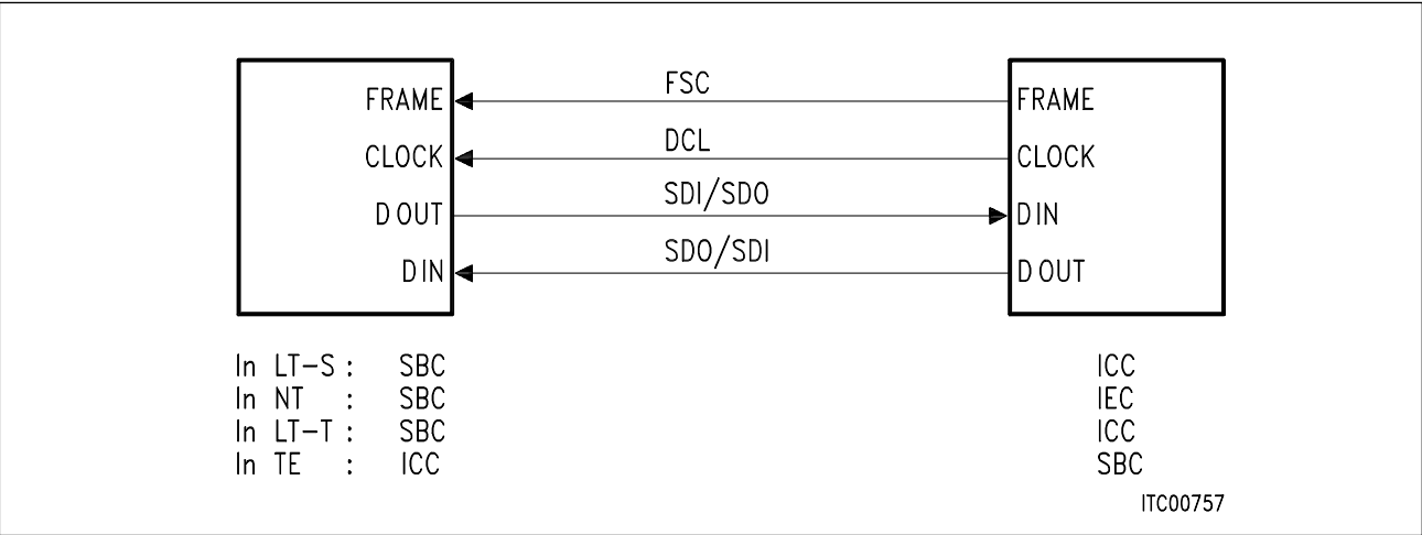
Figure 7 IOM® Interface Signals
