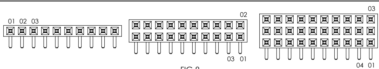
FIG 8 POLARIZATION LOCATION INSERT PK-06-N INTO SPECIFIED POS AND BREAK OFF TAB
