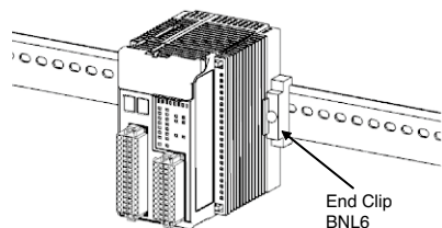
Figure 1. Correct Mounting Direction
