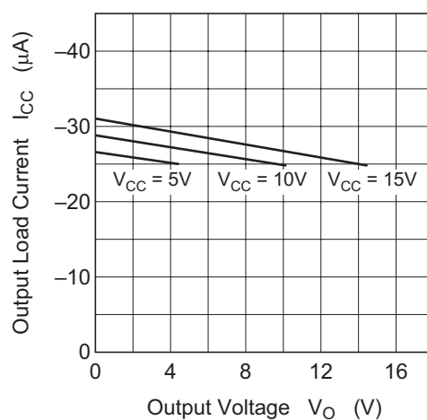
Output Load Current vs. Output Voltage (RNA51957A)
