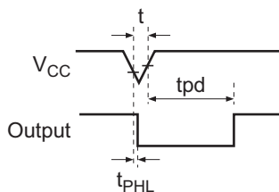
Figure 9 Time Chart at Momentary Voltage-Decrease
