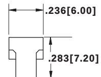
STRAIGHT WITH KINK (SK)
