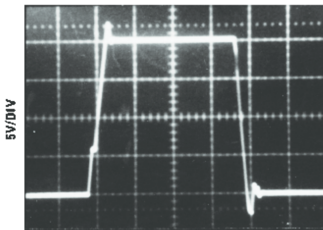
1 \mu s/DIV Figure 38. LF357
