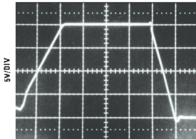
2 \mu s/DIV Figure 36. LF355
