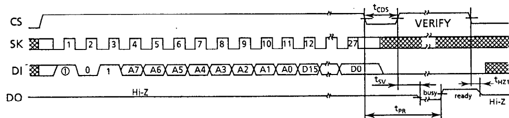
Figure 11 WRITE Timing (S-29331A)
