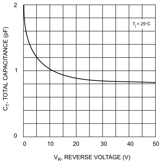
Fig. 5 Typ.Total Capacitance vs Reverse Voltage
