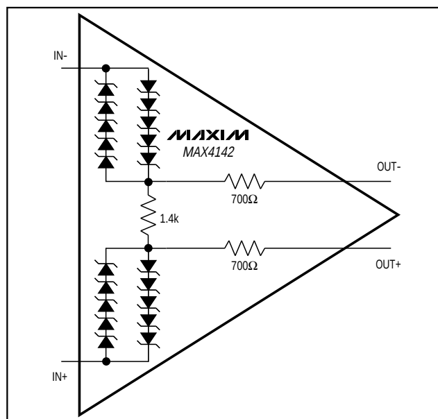
Figure 3. MAX4142 Shutdown Equivalent Circuit
