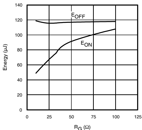
Fig. 15 - Typ. Energy Loss vs. R_G T_J = 175^\circ\text{C} ; L = 1\text{mH} ; V_{CE} = 400\text{V} ; I_{CE} = 4\text{A} ; V_{GE} = 15\text{V}
