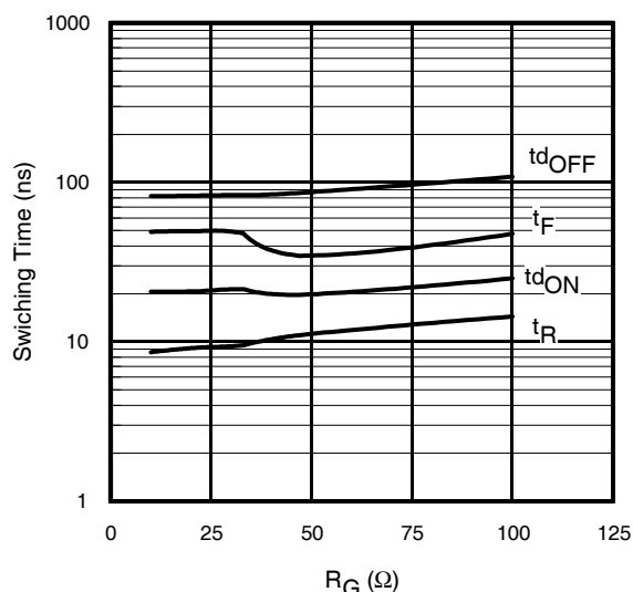
Fig. 16 - Typ. Switching Time vs. R_G T_J = 175^\circ\text{C} ; L = 1\text{mH} ; V_{CE} = 400\text{V} I_{CE} = 4\text{A} ; V_{GE} = 15\text{V}
