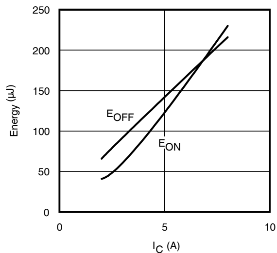
Fig. 13 - Typ. Energy Loss vs. I_C T_J = 175^\circ\text{C} ; L = 1\text{mH} ; V_{CE} = 400\text{V} ; R_G = 100\Omega ; V_{GE} = 15\text{V} .
