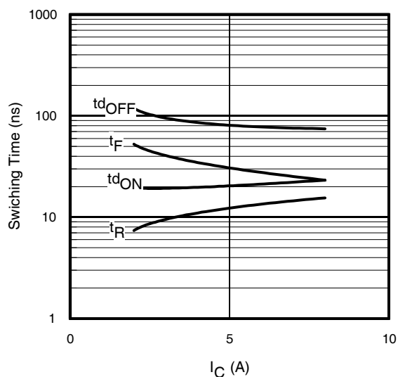
Fig. 14 - Typ. Switching Time vs. I_C T_J = 175^\circ\text{C} ; L = 1\text{mH} ; V_{CE} = 400\text{V} R_G = 100\Omega ; V_{GE} = 15\text{V}
