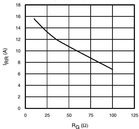
Fig. 18 - Typical Diode I_{RR} vs. R_G T_J = 175^\circ\text{C} ; I_F = 4.0\text{A}
