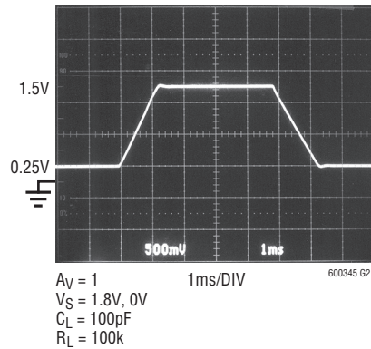
Large-Signal Response
