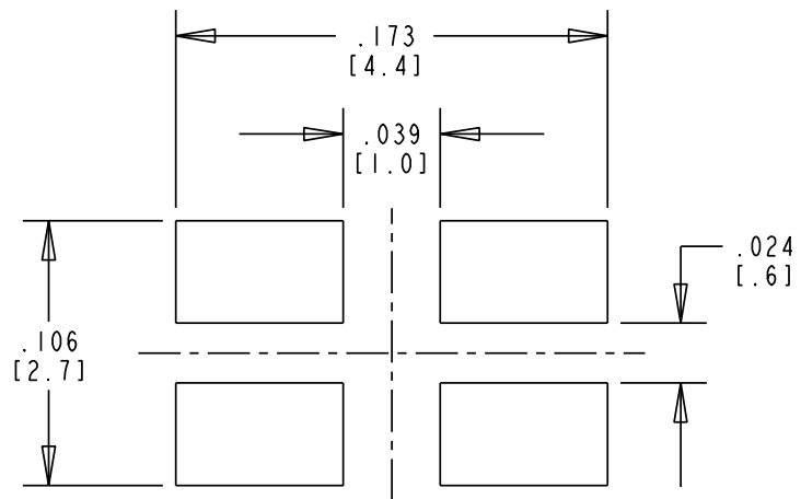
RECOMMENDED SOLDER LAND PATTERN
