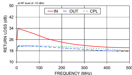
ZFDC-10-1 RETURN LOSS
