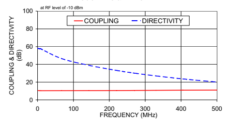
ZFDC-10-1 COUPLING & DIRECTIVITY
