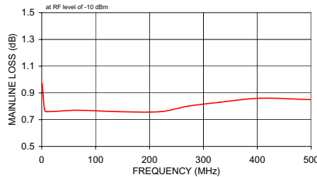
ZFDC-10-1 MAINLINE LOSS
