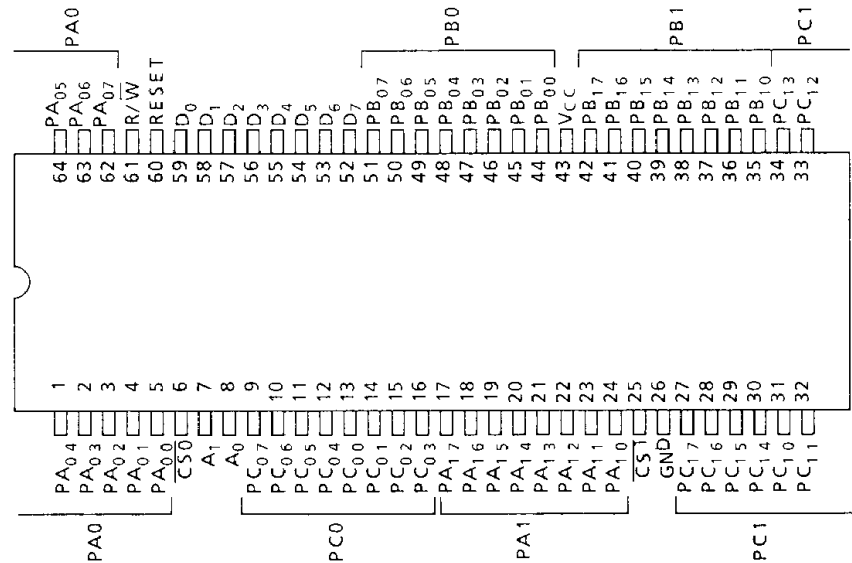
TMP82C265AF-2/TMP82C265AF-10
