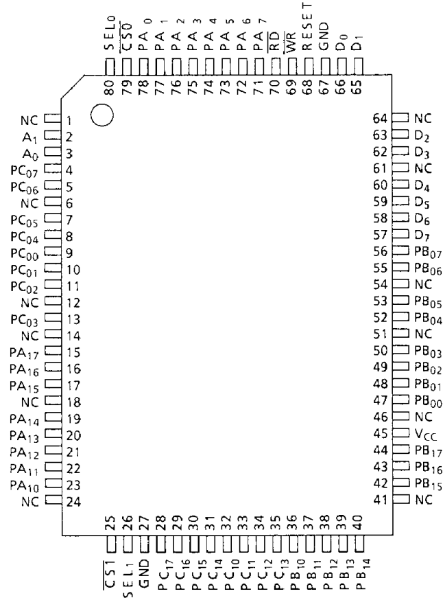
TMP82C265AF-2/TMP82C265AF-10
