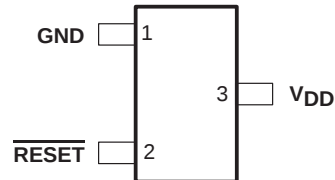
TPS3809 . . . DBV PACKAGE (TOP VIEW)
