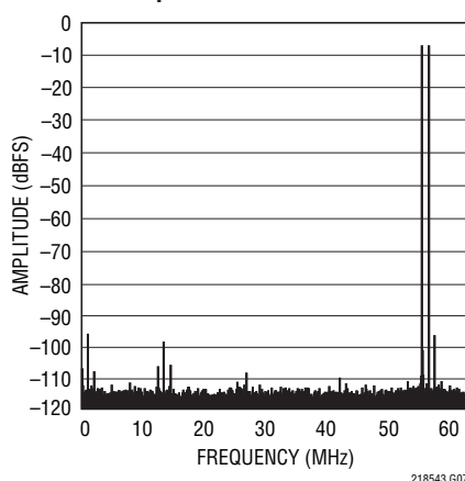
LTC2185: 64k Point 2-Tone FFT, f_{IN} = 69\text{MHz} , 70\text{MHz} , -7dBFS, 125Msps
