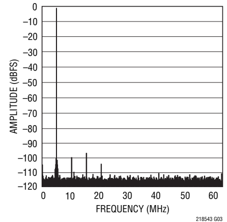
LTC2185: 64k Point FFT, f_{IN} = 5\text{MHz} , -1dBFS, 125Msps
