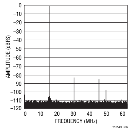
LTC2185: 64k Point FFT, f_{IN} = 140\text{MHz} , -1dBFS, 125Msps
