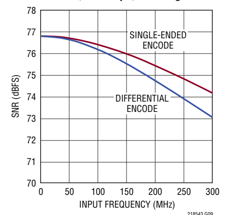
LTC2185: SNR vs Input Frequency, -1dBFS, 125Msps, 2V Range
