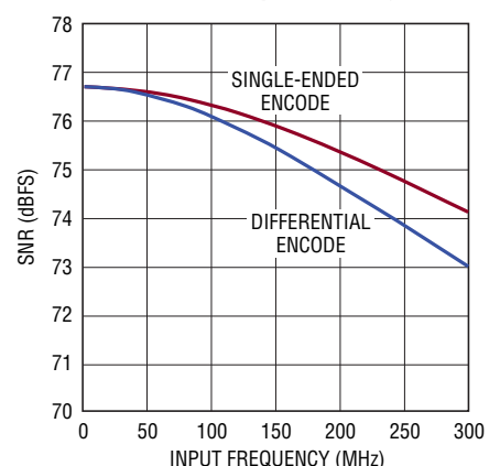
LTC2184: SNR vs Input Frequency, -1\text{dBFS} , 105Mpsps, 2V Range
