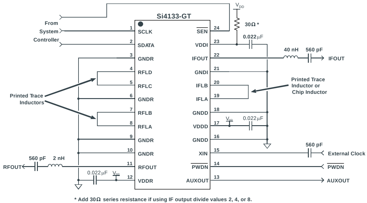
Figure 13. Si4133-GT
