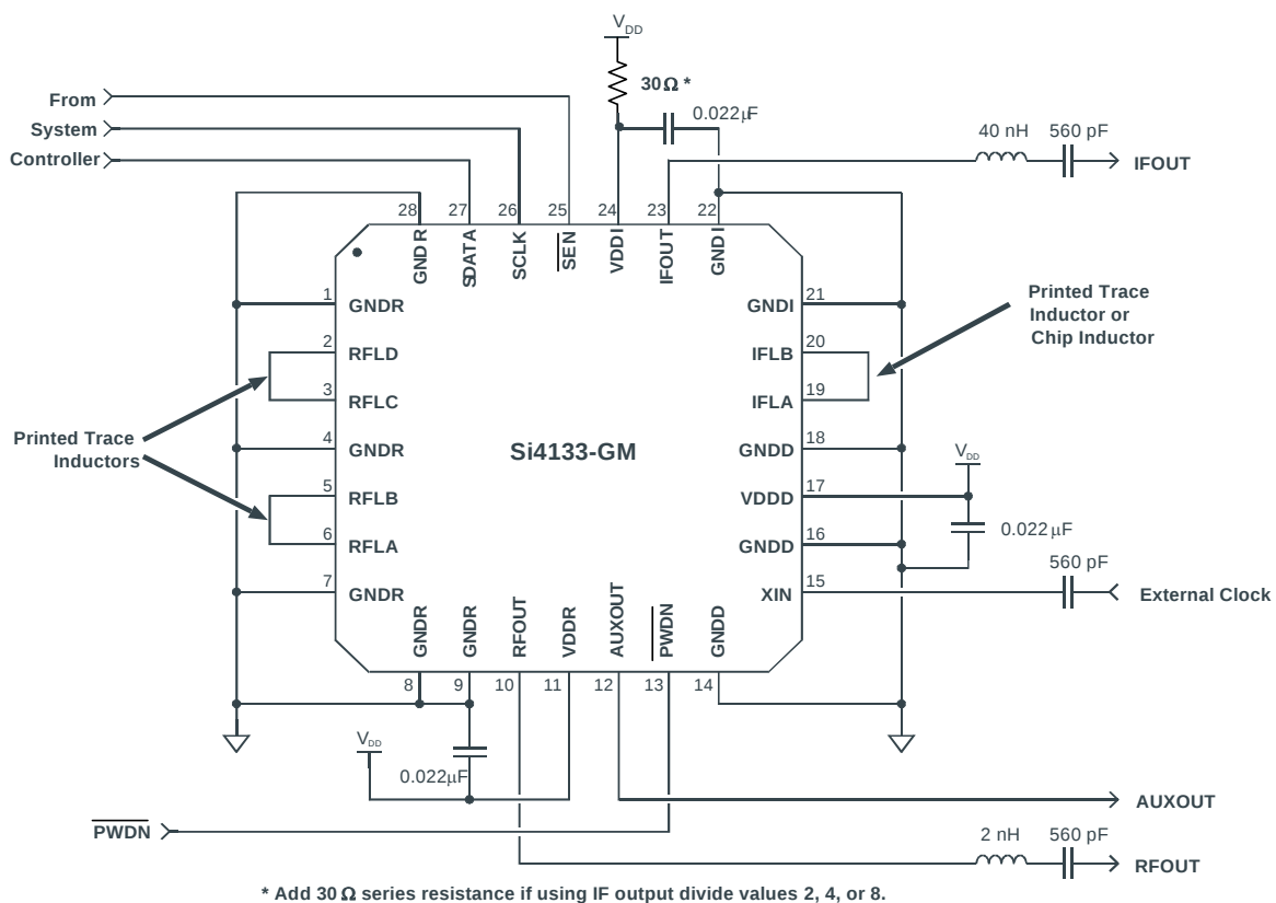
Figure 14. Si4133-GM
