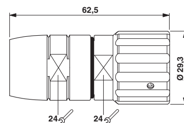
Dimensioned drawing
