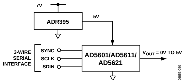
Figure 51. ADR395 as Power Supply to the AD5601/AD5611/AD5621
