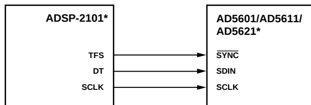
Figure 46. AD5601/AD5611/AD5621 to ADSP-2101 Interface
