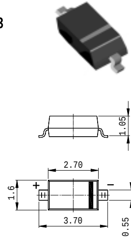
SOD-123
