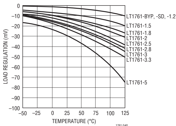
Load Regulation \Delta I_L = 1\text{mA} to 100mA
