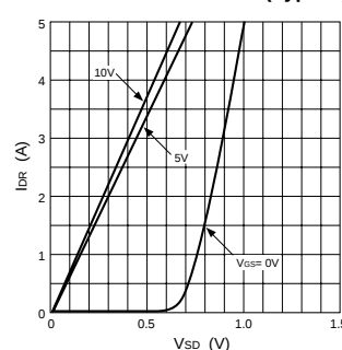
I DSR -V SD Characteristics (Typical)
