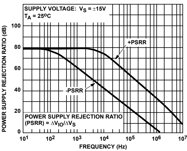
FIGURE 36. POWER SUPPLY REJECTION RATIO vs FREQUENCY
