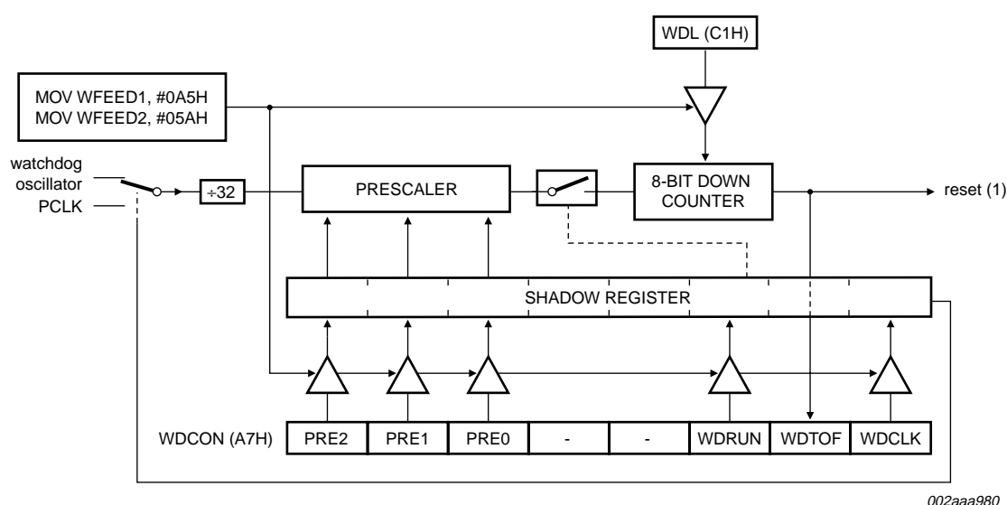
Fig 17. Watchdog timer in Watchdog mode (WDTE = 1)
