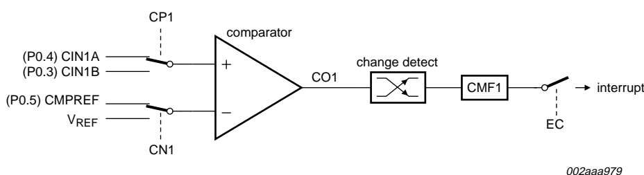
Fig 16. Comparator input and output connections
