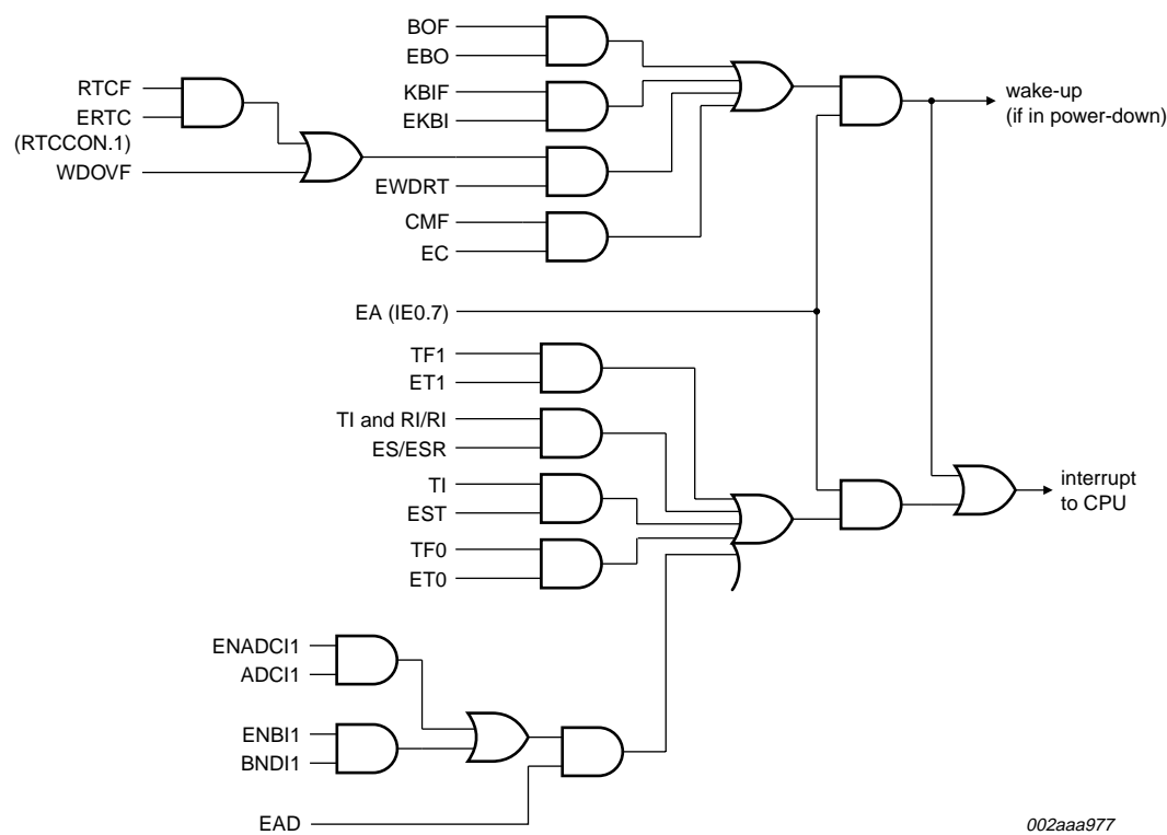
Fig 14. Interrupt sources, interrupt enables, and power-down wake-up sources (P89LPC9103/9107)
