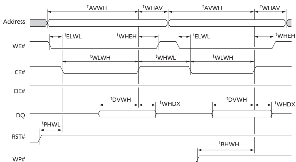
Figure 23: Write-to-Write Timing
