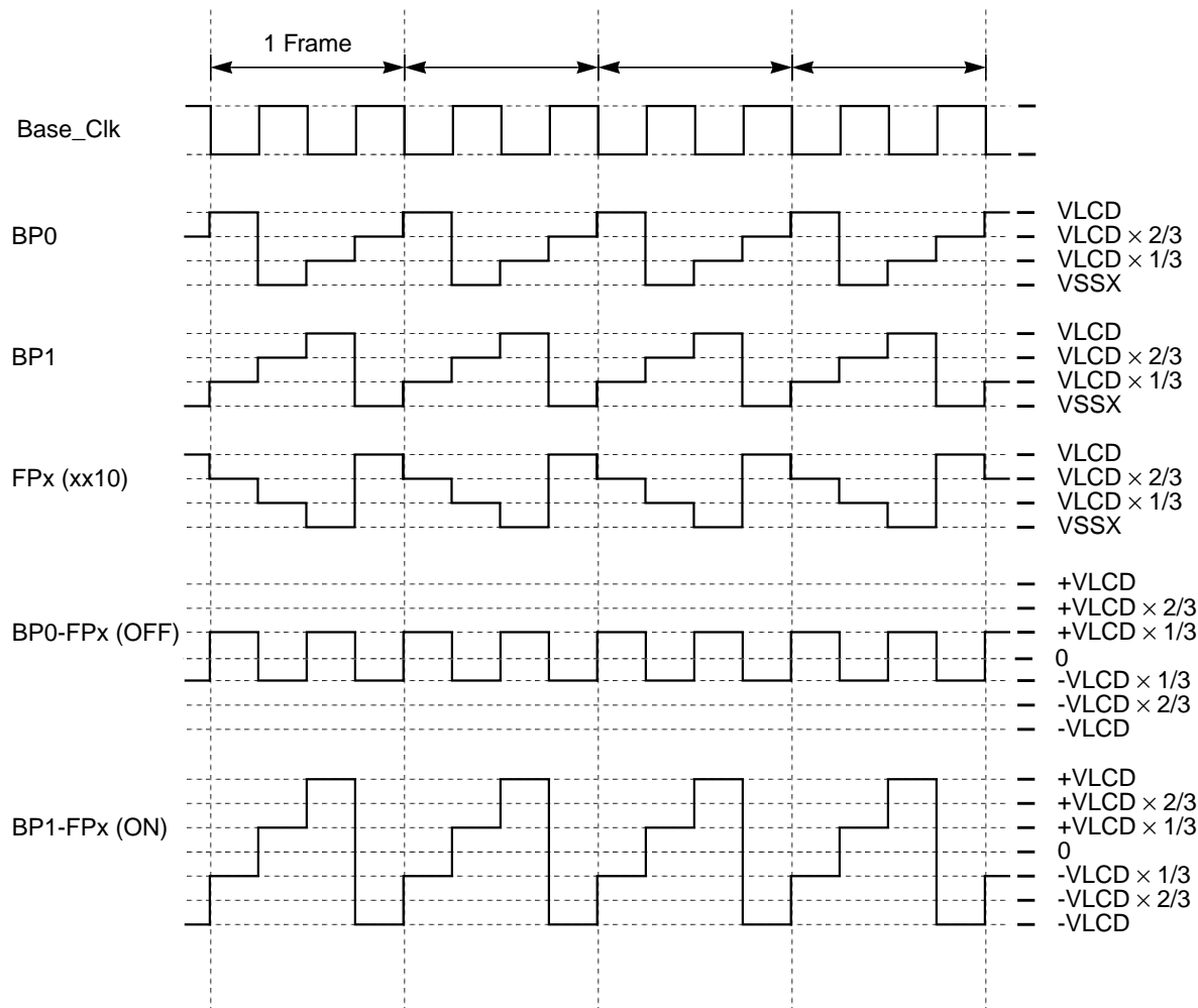
Figure 9-11. 1/2 Duty and 1/3 Bias (Normal Waveform)
