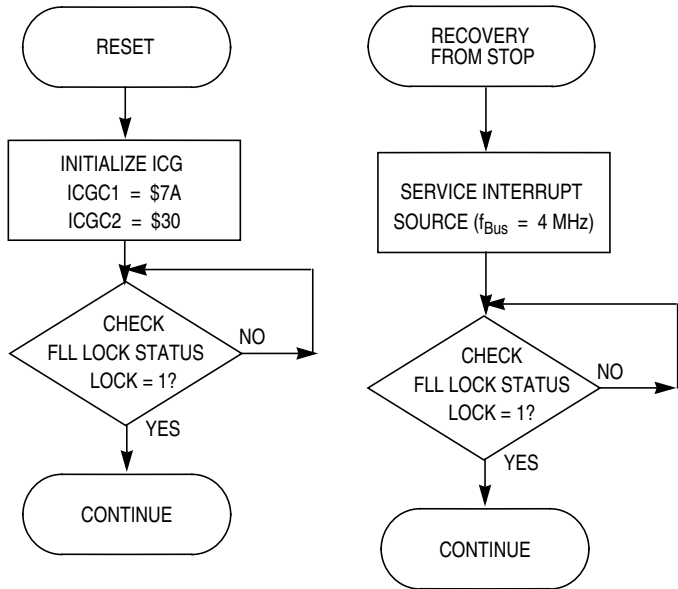
Figure 10-15. ICG Initialization and Stop Recovery for Example #2
