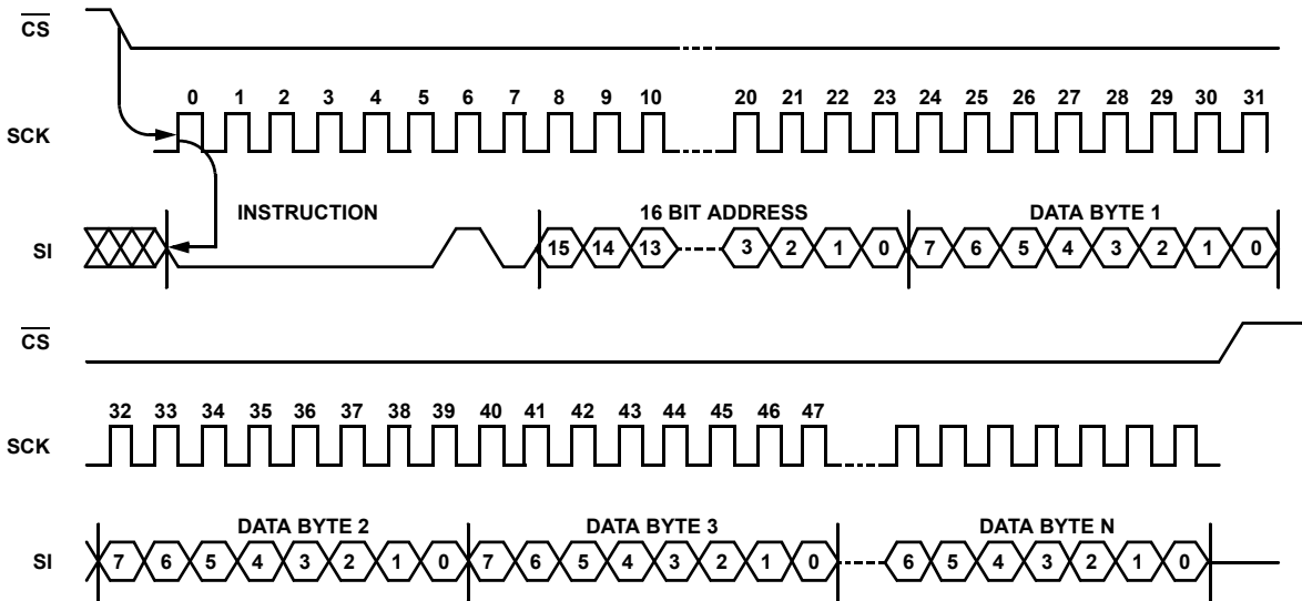
FIGURE 8. WRITE SEQUENCE
