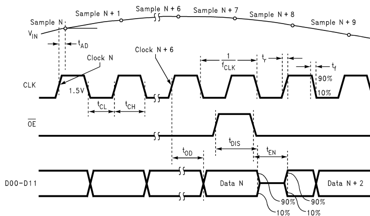
Figure 1. Output Timing
