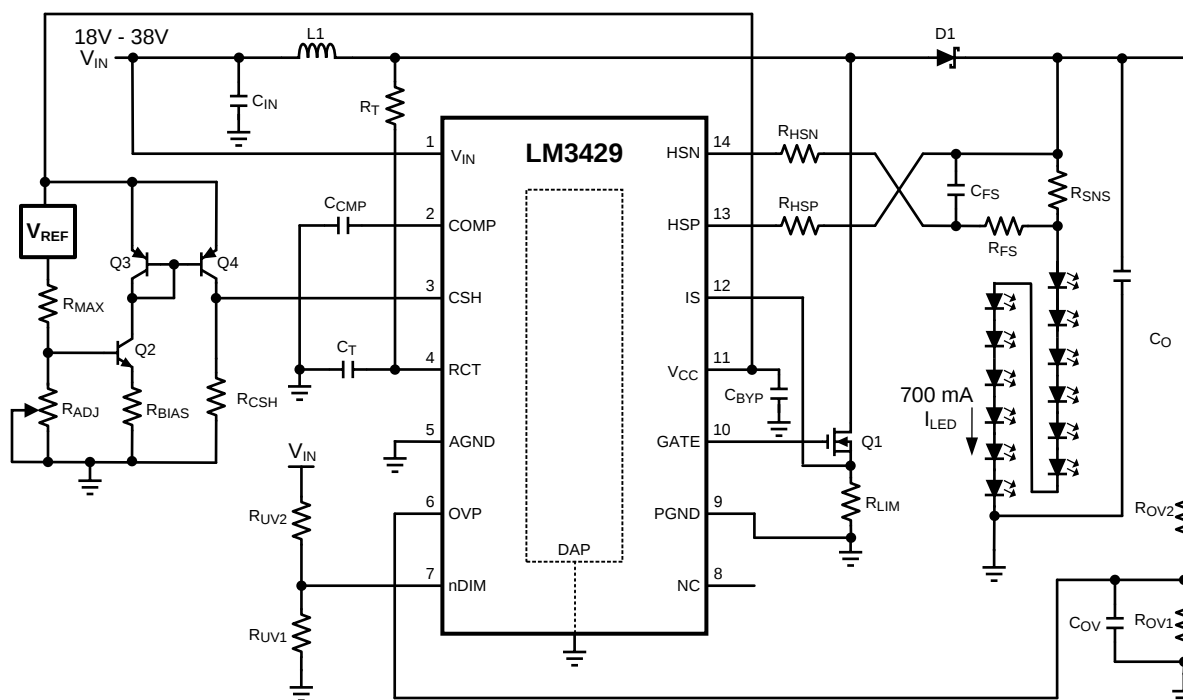
Figure 33. Boost Analog Dimming Application - 12 LEDs at 700 mA Schematic
