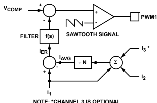
FIGURE 6. CHANNEL-1 PWM FUNCTION AND CURRENT-BALANCE ADJUSTMENT
