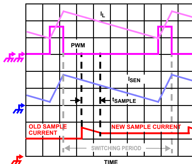
FIGURE 3. SAMPLE AND HOLD TIMING
