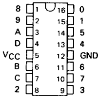
J OR N PACKAGE (TOP VIEW)
