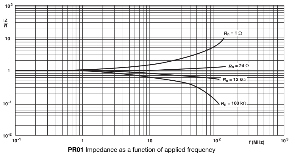
PR01 Impedance as a function of applied frequency
