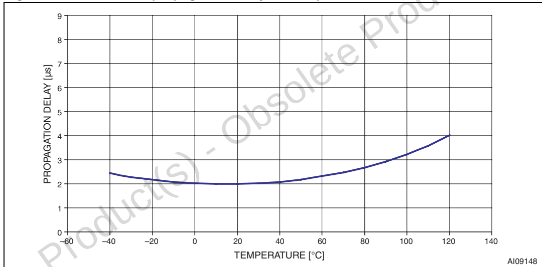
Figure 17. PFI to \overline{PFO} propagation delay vs. temperature
