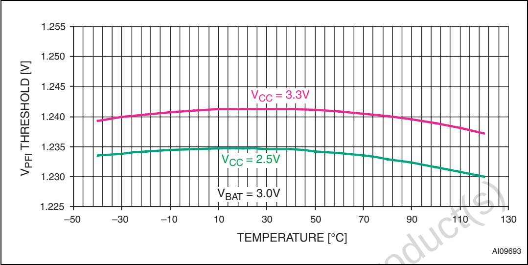
Figure 13. V_{PFI} threshold vs. temperature
