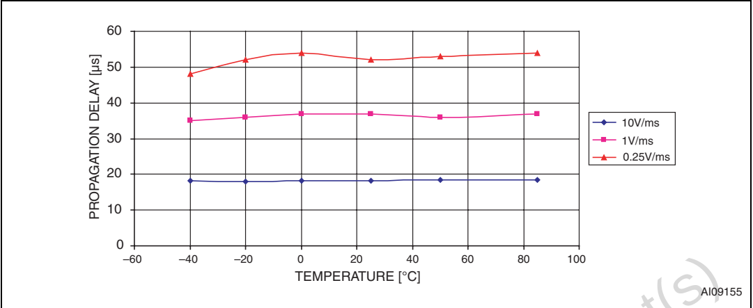
Figure 22. V_{CC} to reset propagation delay vs. temperature
