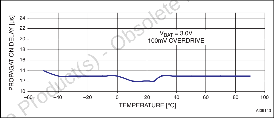
Figure 14. Reset comparator propagation delay vs. temperature
