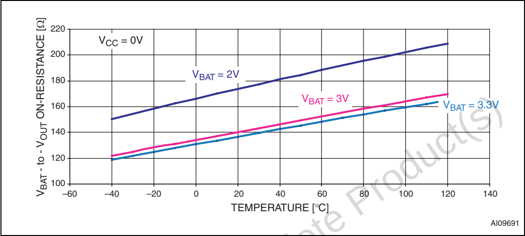
Figure 11. V_{\text{BAT}} -to- V_{\text{OUT}} on-resistance vs. temperature
