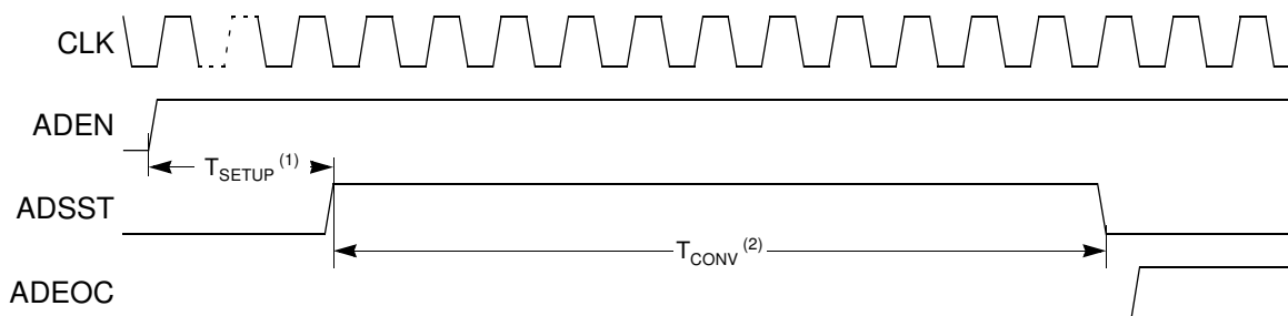
Figure 46. Timing Diagram
