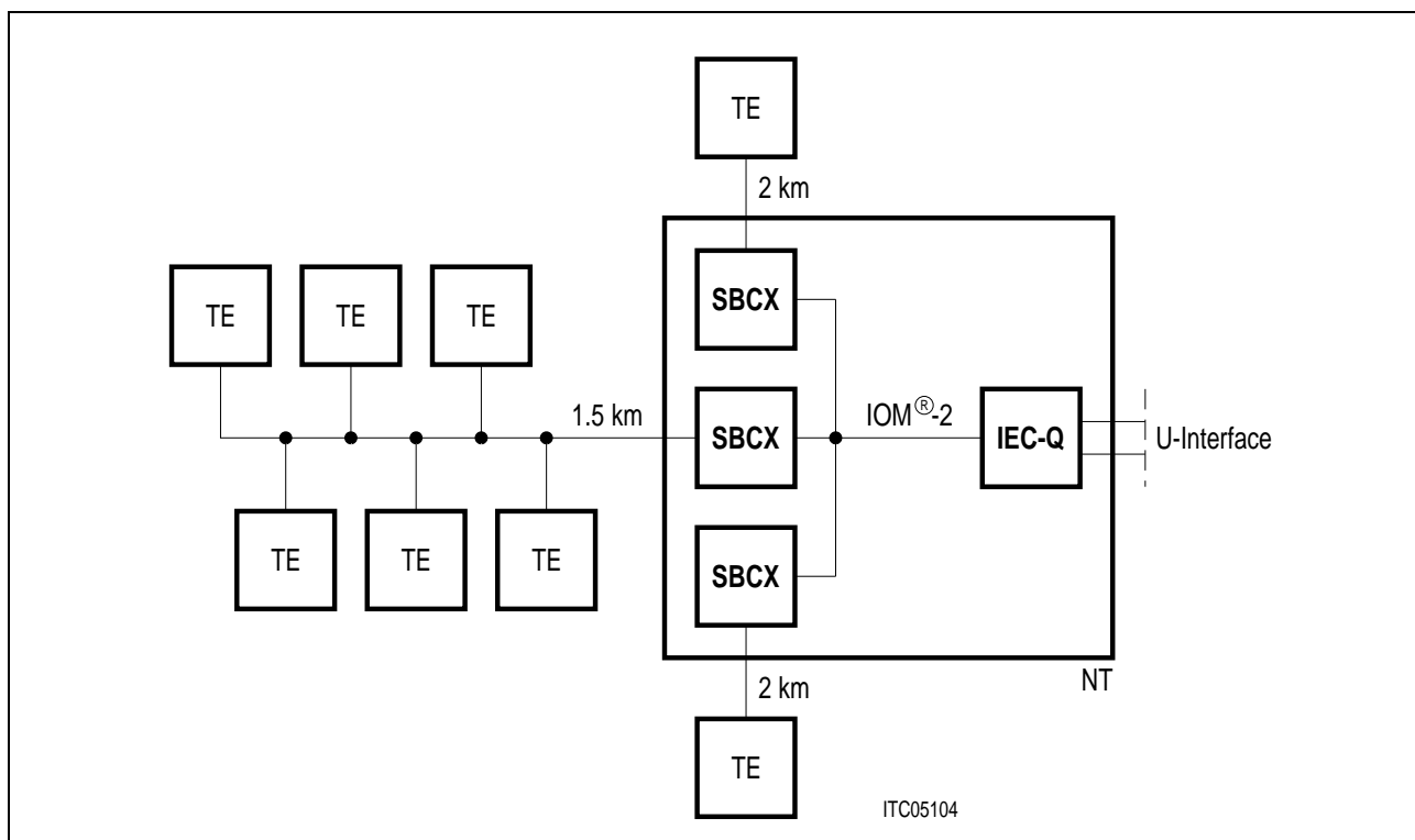
Figure 10 NT-Star Configuration with 2 TEs Connected Point-to-Point and 6 TEs Connected via an Extended Passive Bus
