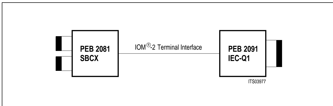
Figure 7 Basic Network Terminator (NT1)
