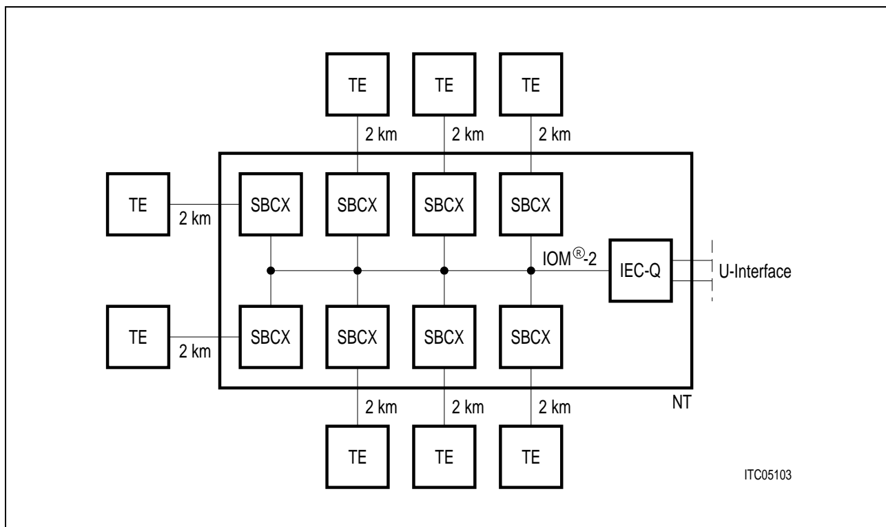
Figure 9 NT-Star Configuration with 8 TEs Connected Point-to-Point
