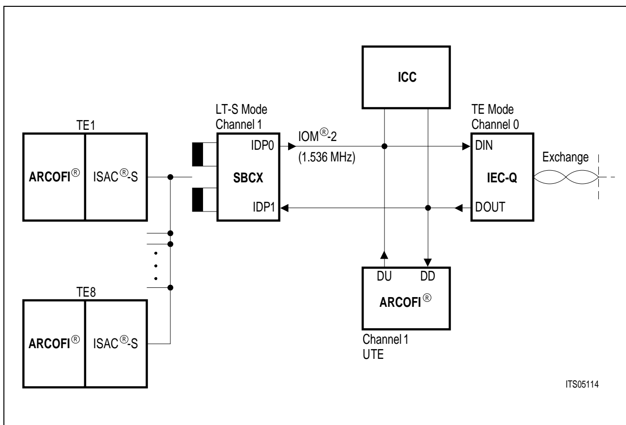
Figure 43 Intelligent NT-Configuration for IOM ® -2 Channel Switching
