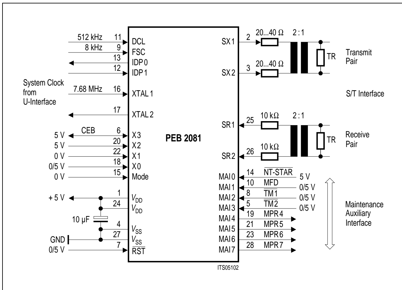
Figure 8 SBCX in NT-Mode
