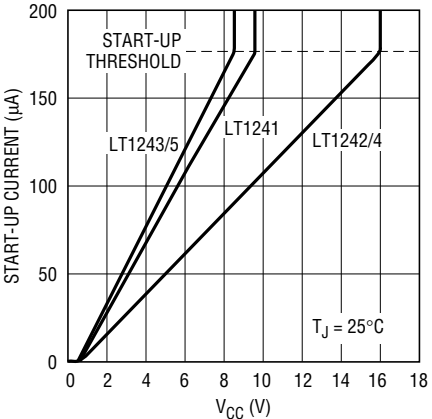
Start-Up Current
