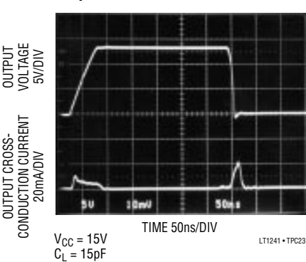
Output Cross-Conduction Current
