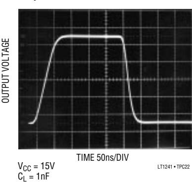
Output Rise and Fall Time
