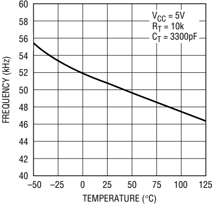
Oscillator Frequency
