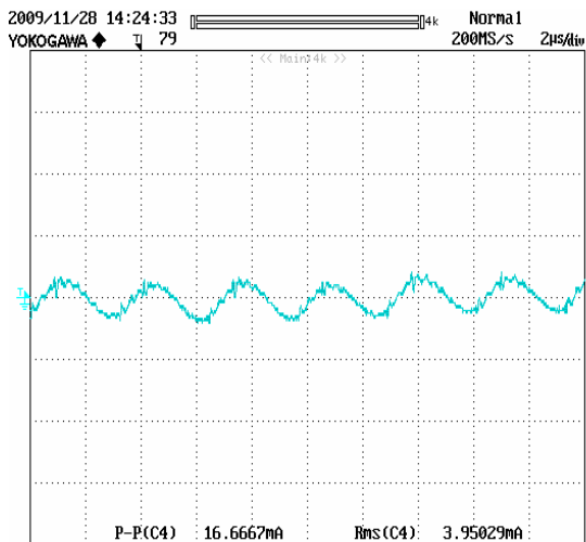
Figure 12: Input reflected ripple current, i_s , through a 12\mu\text{H} source inductor at nominal input voltage and rated load current (20 mA/div, 2us/div).
