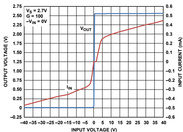
Figure 19. Input Overvoltage Performance, Single Supply, V_S = 2.7V , G = 100
