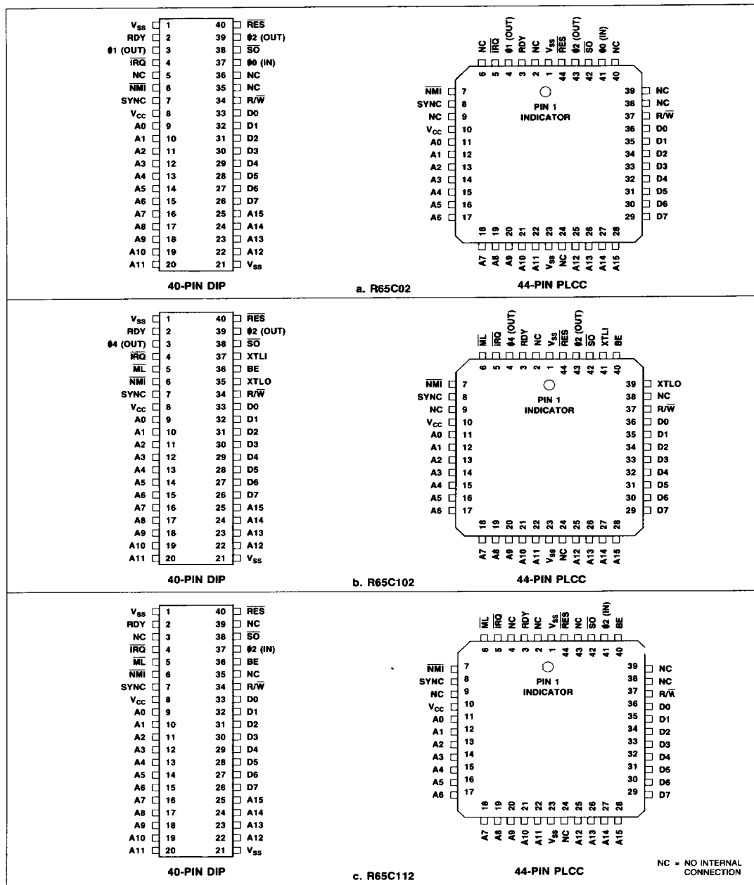
Figure 1. Pin Assignments
