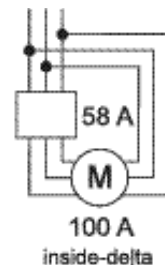
In-line and inside-delta connection of PS S 18/30...300/515
