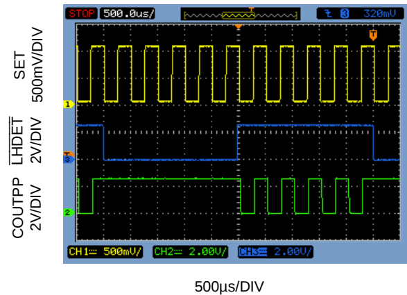
COUTPP Transient Response with \overline{LHDET} V_{IN} = OV_{DD} = 2.5V , C_{LOAD} = 15pF
