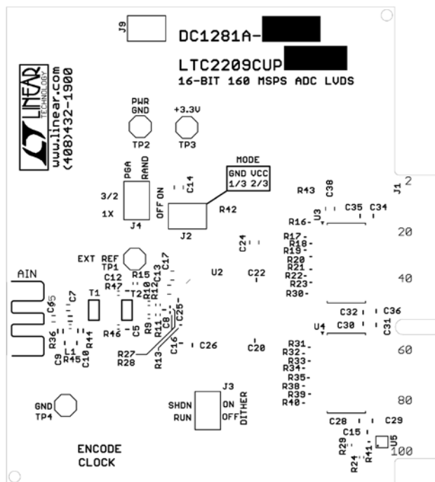
Silkscreen Top
